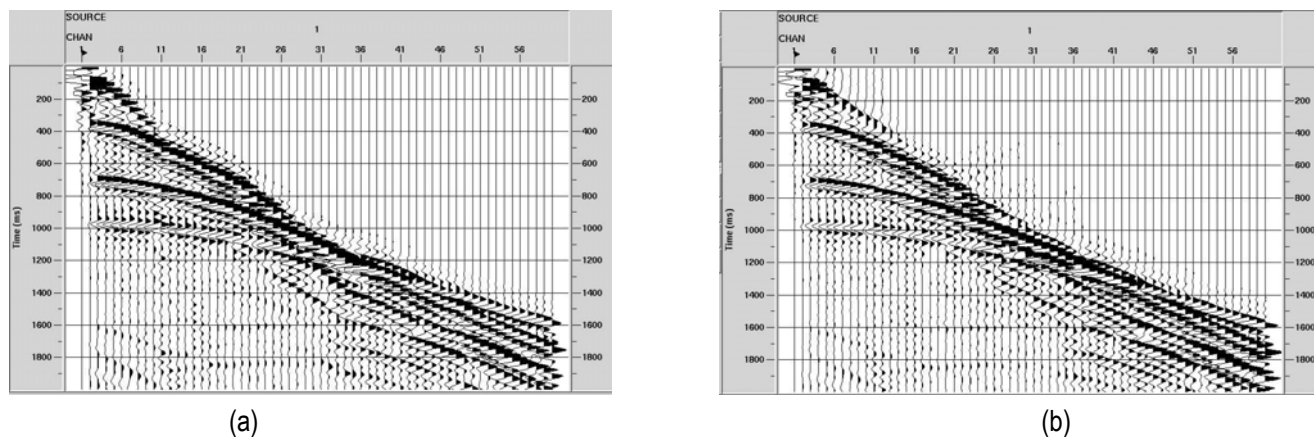
Figure 5. (a) After applying vertical static shifts to move the data to a flat datum. (b) After wave equation datuming. Note that wave equation datuming result is superior to the vertical static shifts where raypaths are not near the vertical (Case II).
