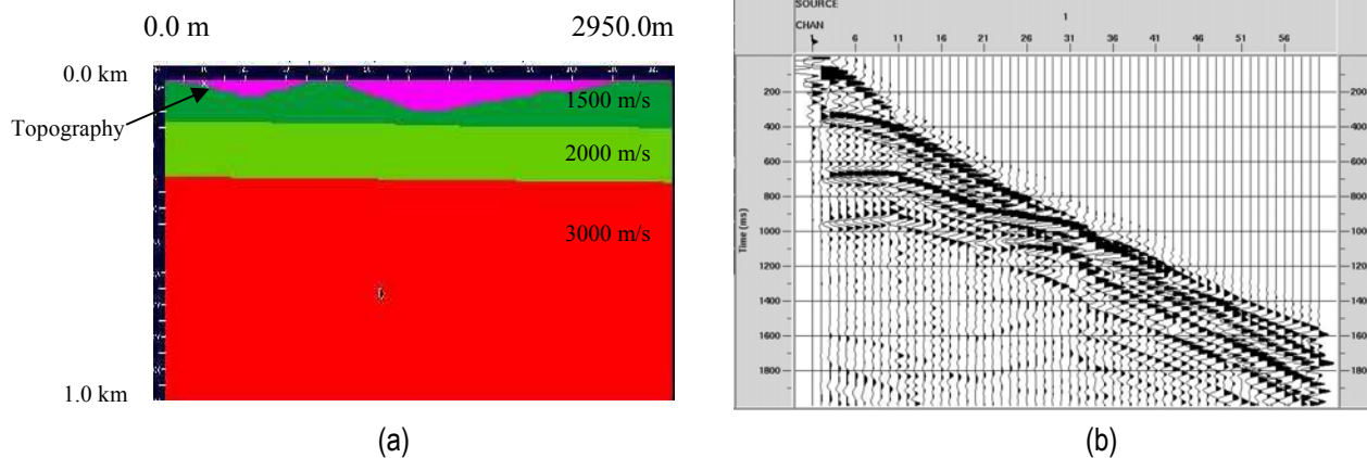
Figure 4. (a) Velocity model used for case II. (b) The synthetic shot gather for this model.
