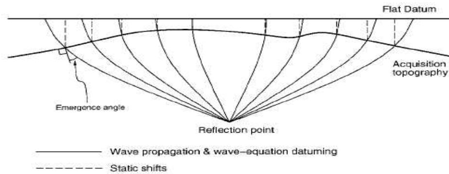
Figure 1. A comparison between wave equation datuming and vertical static shifts (taken from Bevc (1997)).
