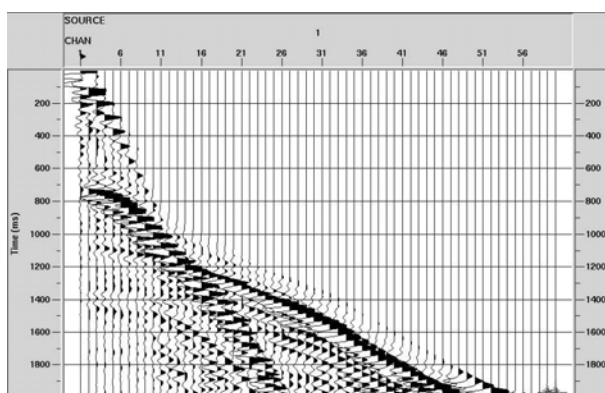
Figure 3. (a) After applying vertical static shifts to move the data to a flat datum. (b) After wave equation datuming. Both have resolved most of the topography related statics. These results are for Case I.
