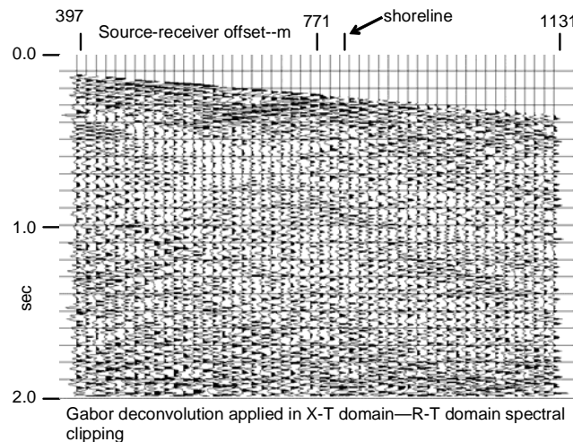
Fig. 8. Source gather from Figure 7 after the additional step of Gabor deconvolution whitening. Underlying reflections much more visible.
