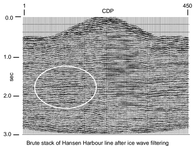
Fig. 10. Hansen Harbour line after R-T domain ice wave attenuation. Reflection continuity improved at all levels.
