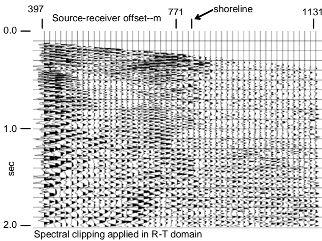
Fig. 7. Source gather from Figure 1 after spectral clipping in the R-T domain. Ice wave residual still visible, but much diminished.
