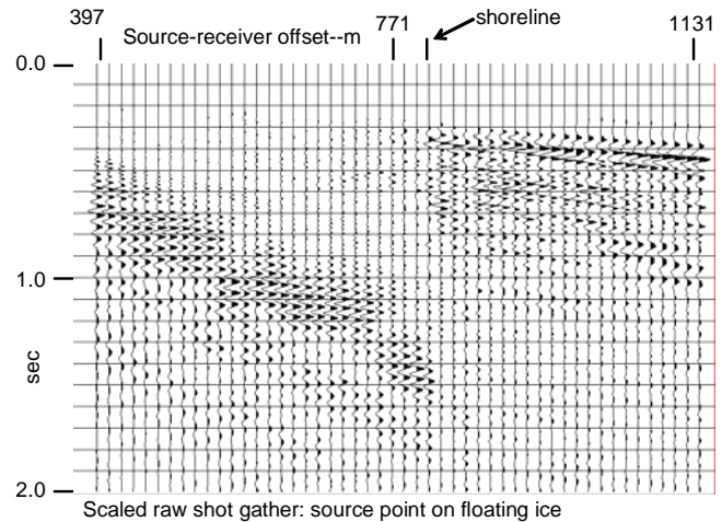
Fig. 2. Raw source gather from Hansen Harbour, source on floating ice. Trace amplitudes normalized.
