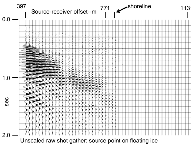
Fig. 1. Raw source gather from Hansen Harbour, source on floating ice. Relative trace amplitudes preserved.
