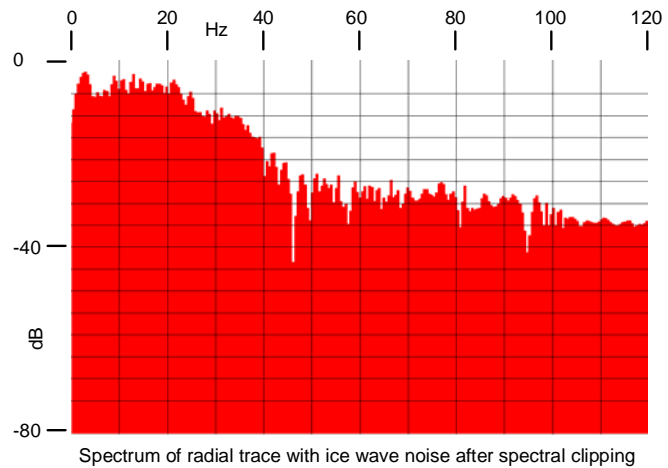
Fig. 6. Spectral clipping eliminates monochromatic spectral peaks, leaving background signal spectrum relatively unaffected.
