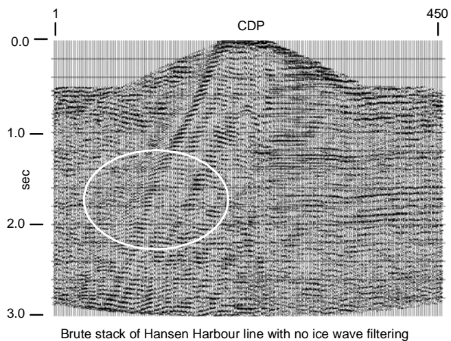
Fig. 9. Brute stack of the vertical component of the Hansen Harbour 3-C experimental line—no coherent noise attenuation.
