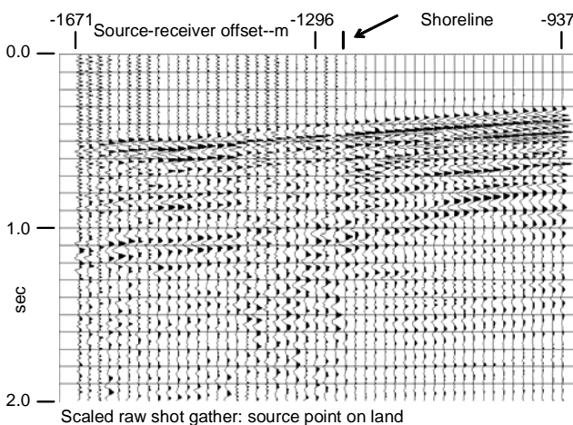
Fig. 3. Raw source gather from Hansen Harbour, source on land. Trace amplitudes normalized. Reflections seen even on geophones planted on floating ice.
