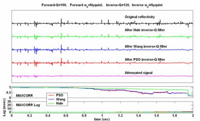
Figure 6. Same experiment as in figure 5, but for Q=100 . Hale filter shows a considerable advantage over the other two methods in recovering amplitude. The amplitude recovery in the three methods is practically perfect as can be observed in the MAXCORR lag curve which is practically zero for any method.
