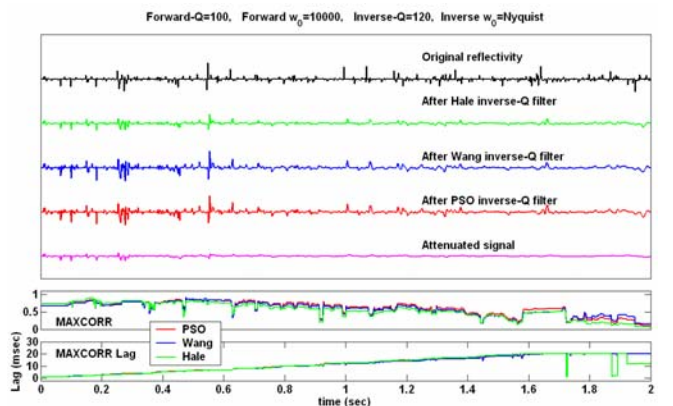
Figure 8. Same experiment as in figure 6, but for Q=100 . PDO method becomes the best in recovering amplitude, followed by Wang. Hale method may become the worst method in recovering amplitude when considering uncertainty in Q and \omega_0 , as in this case.
