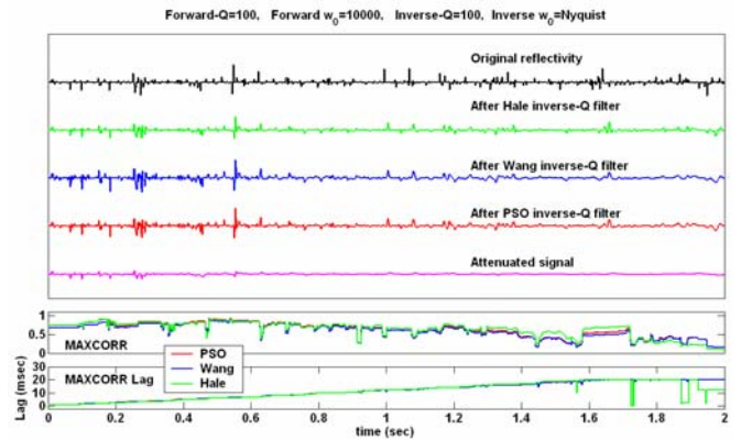
Figure 4. Same experiment as in figure 3, but for Q=100 . Hale filter has lost its huge advantage over the other two methods. The amplitude and phase recovery of the three methods is similar. The growing phase lag due to the pedestal effect remains in the trace after applying inverse-Q filter using any method.
