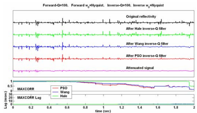
Figure 2. Same experiment as in figure 1 for Q=100. The same trends observed in the previous figure can be observed here, although the amplitude recovery has improved in Wang and PDO methods with respect to the case for Q=50, as can be easily observed by comparing the MAXCORR curve in both experiments.
