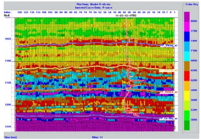
FIG. 2. Results of the model-based P-impedance inversion
