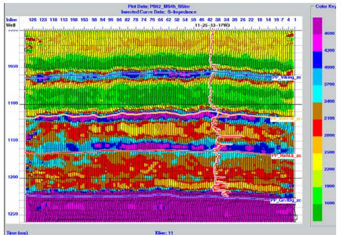
FIG. 5. The inversion result of PS data.
