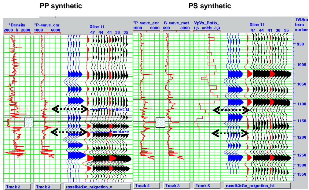
FIG. 7. PP and PS synthetic seismograms and seismic traces.
