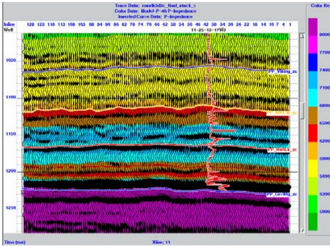
FIG. 1. The P-impedance model with P-impedance log inserted.
