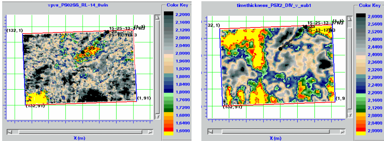
FIG. 6. Comparison of Vp/Vs derived from impedance (left) and Vp/Vs derived from time-thickness ratios (right).
