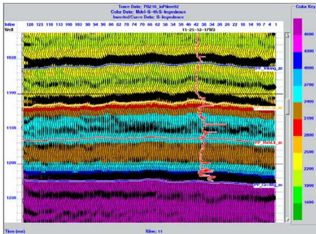
FIG. 4. The S-impedance background model.
