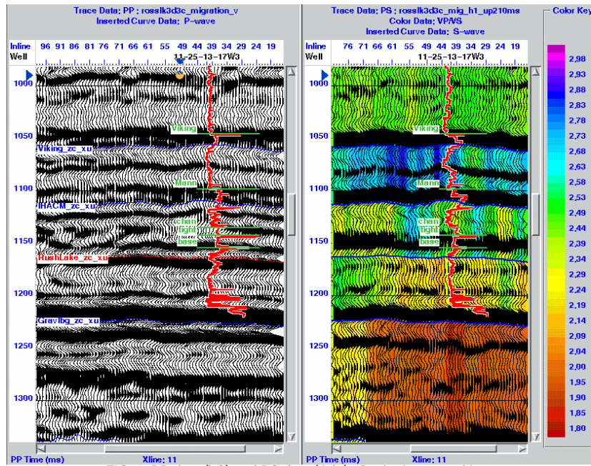
FIG. 3. PP data (left) and PS data (right) after horizon-matching.
