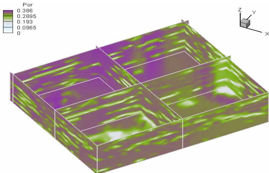
Figure 1 3-D visualization of the porosity model
