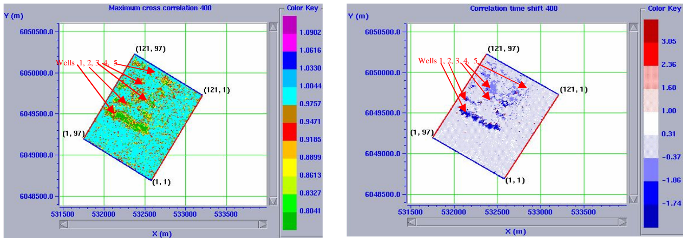
Figure 5 Cross correlation coefficient (left) and time shift (right) of seismic traces between the baseline survey and the monitor survey
