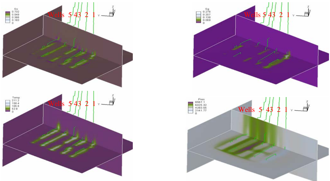
Figure 2 Distribution of oil saturation (upper left), gas saturation (upper right), temperature (lower left) and pressure (lower right) at the end of February, when the first monitor seismic survey was shot in an attempt to monitor the fluid flow.
