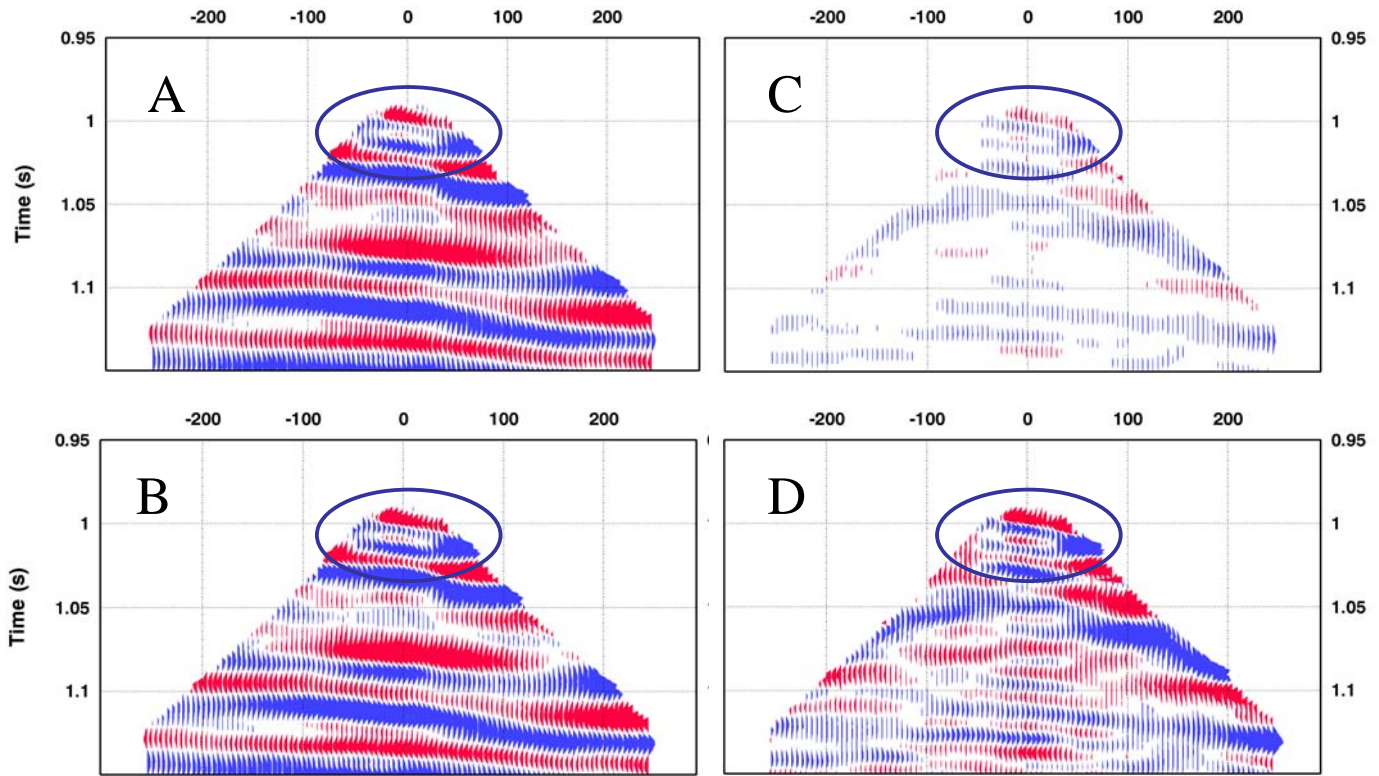
Figure 5: Comparison of the baseline and monitor migrated images from Line 2. The Cardium is located at the top of the image. A is the baseline, B is the monitor, C is the difference between the monitor and the baseline, and D is the difference display with the amplitudes scaled up 4 times.
