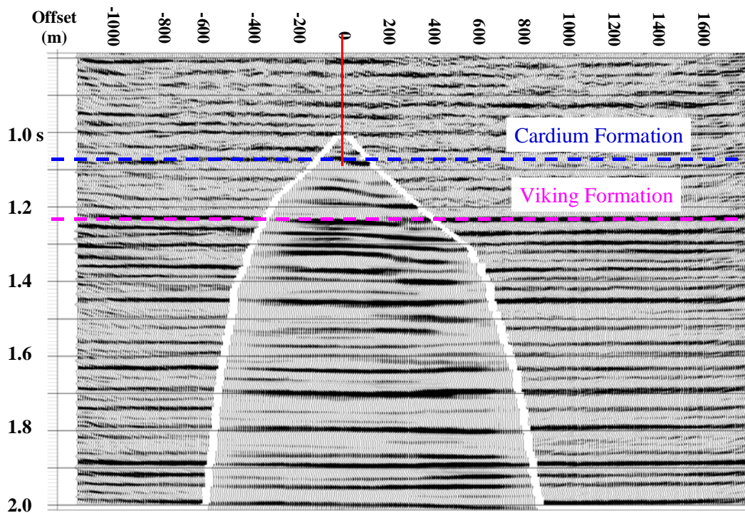
Figure 3: Comparison of the baseline P-wave surface and borehole seismic data for Line 3.
