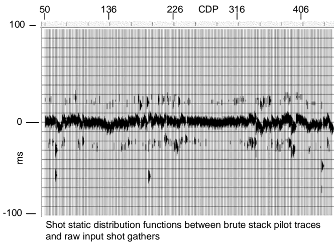
FIG. 4. The distribution functions estimated for Hansen Harbour line
