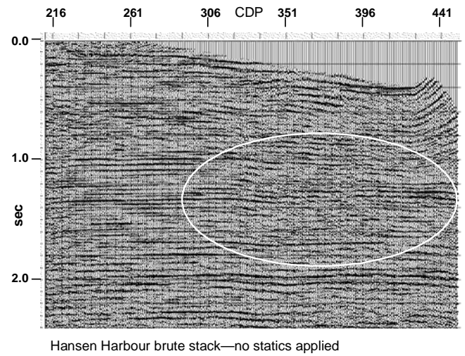
FIG. 6. Hansen Harbour brute stack—no statics
