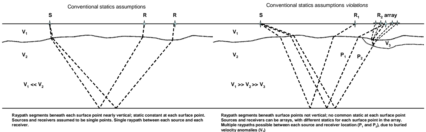
FIG. 1. Simplifying assumptions for surface-consistent statics FIG. 2. Surface-consistency violated in several ways.
