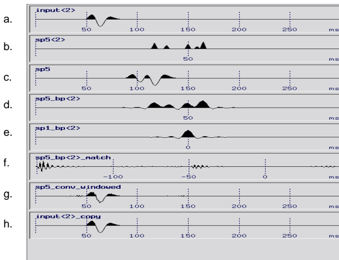
The static deconvolution principle
