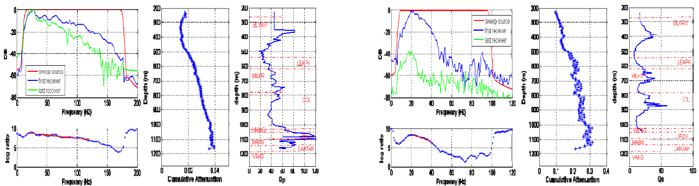
Figure 2: left, - amplitude spectrum and spectral ratio (sweep source in red, the first depth level in blue and the bottom receiver in green); cumulative attenuation calculated from the spectral ratio method; and estimated interval Q values of P wave. The right plots are for the shear wave.
