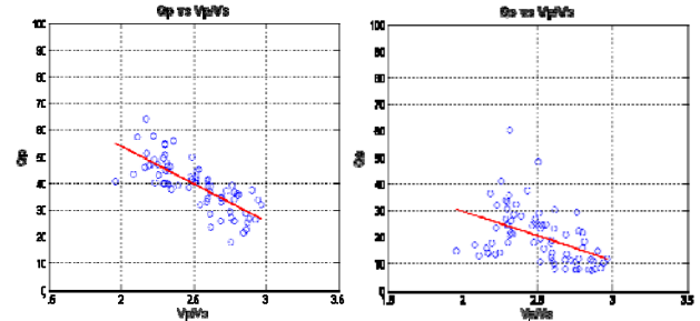
Figure 6: Crossplot between Q_p and V_p/V_s (left) and Q_s vs. V_p/V_s (right).
