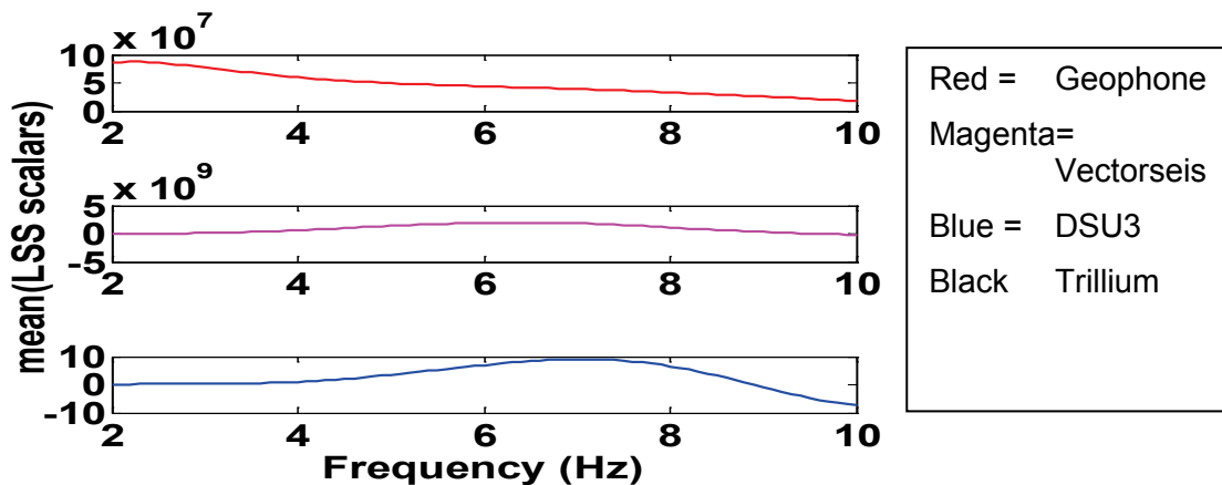
Figure 4. Averaged LSSS for all sensors and for all 2-10 Hz sweeps.
