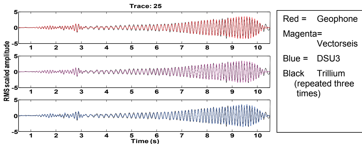
Figure 2. Vertical component uncorrelated traces from 50 m south of the north SP for a 10 s 2-10 Hz sweep.
