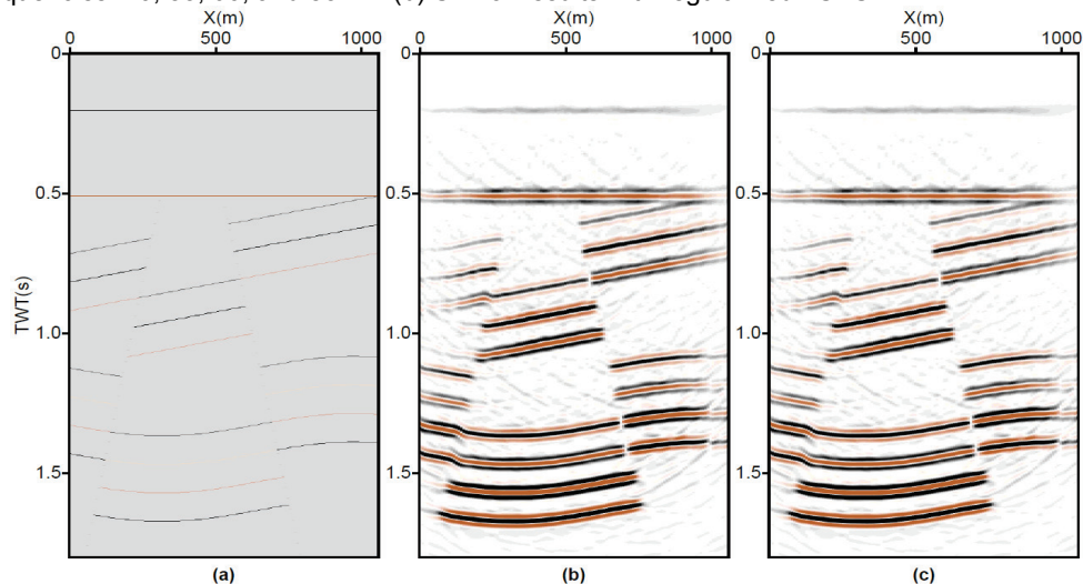
Figure 3. Comparison between true model (a), CGLS (b), and Multigrid CGLS (c) of a synthetic seismic dataset.
