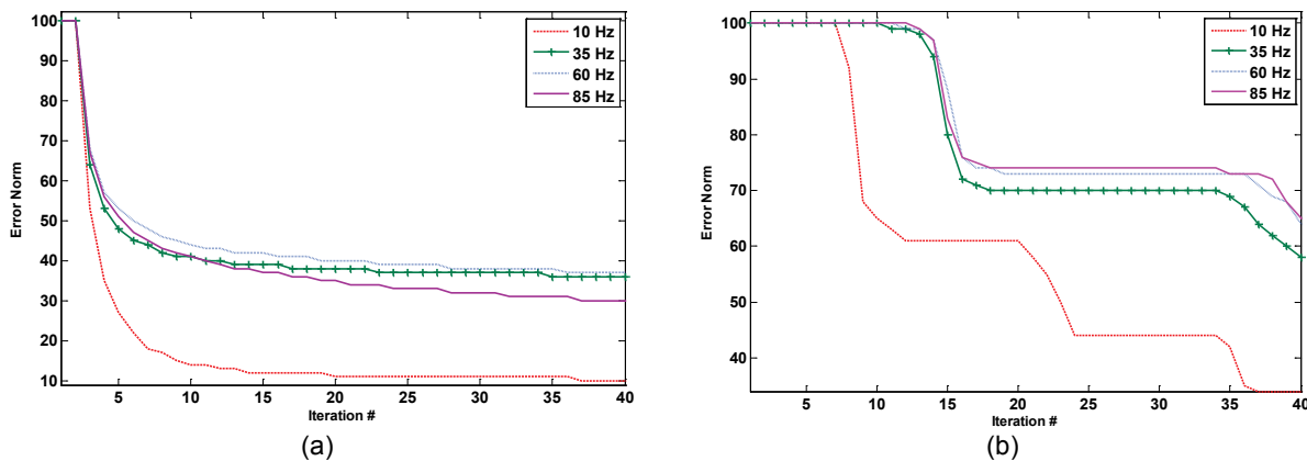
Figure 2. (a) Convergence of CGLS to solve damped LSPSTM for a synthetic model with wavelets having different dominant frequencies: 10, 35, 60, and 85 Hz. (b) Similar results with regularized LSPSTM.
