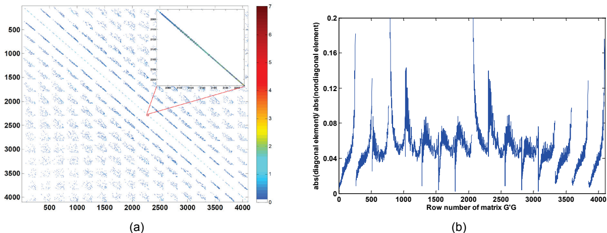
Figure 1. (a) Non-zero elements of matrix G'G . (b) The ratio of absolute values of diagonal elements to the sum of absolute values of nondiagonal elements for each row of G'G . Values higher than 1 are diagonally dominant rows.
