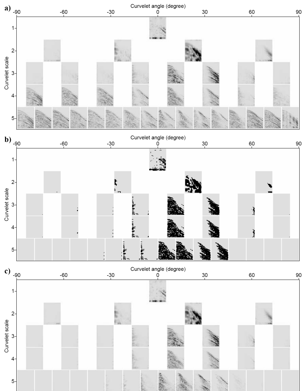
Figure 3 a) Curvelet domain representation of the data from Figure 2a after pre-processing (interlacing 7 zero traces between each available traces). b) Mask function computed from (a) using thresholding for scales 1 to 3. The mask function for scales 4 and 5 were bootstrapped from scale 3 following the algorithm discussed in the text. c) Curvelet coefficients of the interpolated data.
