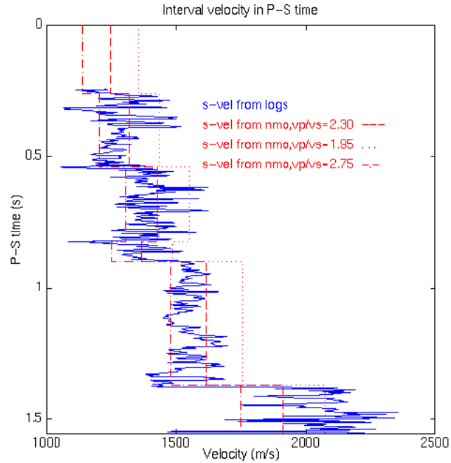
Fig. 6. Comparison of Dix estimates from the velocity analysis of figure 5 to the S-wave well log. The different \gamma values (1.95 and 2.75) around 2.3 change the \beta estimates by about 10%.
