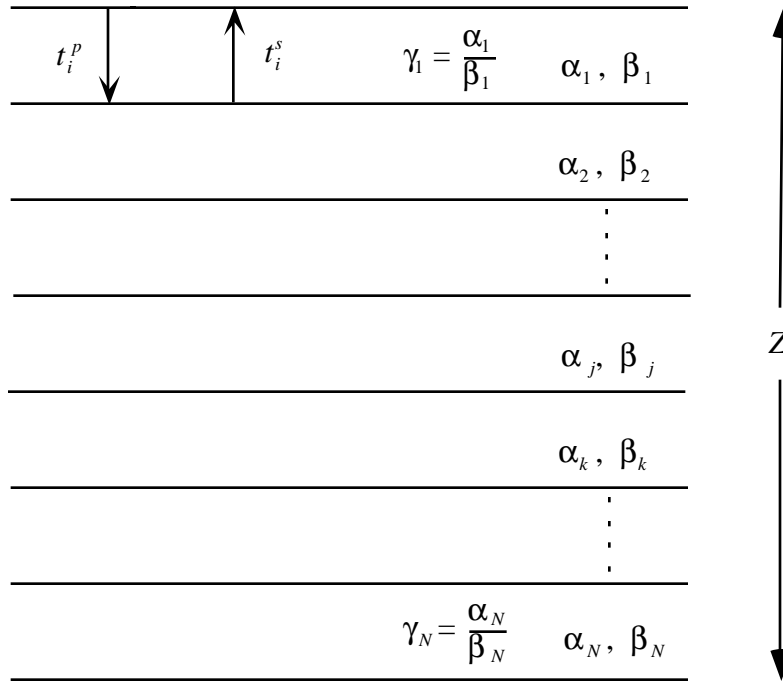
Fig. 1. Plane-layer elastic medium with N layers.
