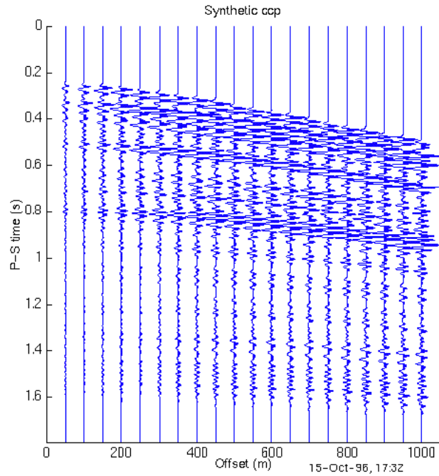
Fig. 4. Synthetic seismic data from the SYNTH, (P-S component). Offsets 0 - 1000 m are shown here. The range of offsets used in velocity analysis (Figure 5) extended from 0m to 2500m.
