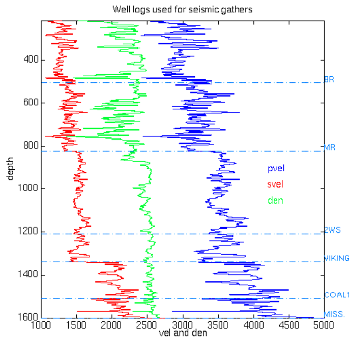
Fig. 2. Logs used to generate the P-S gather of Figure 4. The S-wave velocity (left) was derived from the P-wave velocity (right) using a depth varying V_p/V_s (Figure 3).
