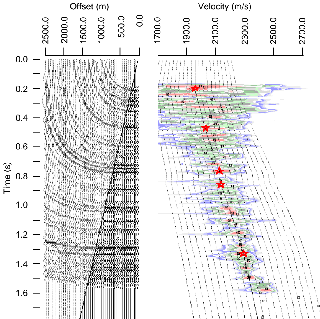
Fig. 5. Semblance velocity analysis of the P-S gather. The gather is shown with the stacking velocity applied (left). The stacking function is marked by stars (right). Note the offset mute required to obtain event flattening (stretch mute = 10%) at near offsets. AGC has been applied to enhance the amplitude of the near offsets to further improve semblance.
