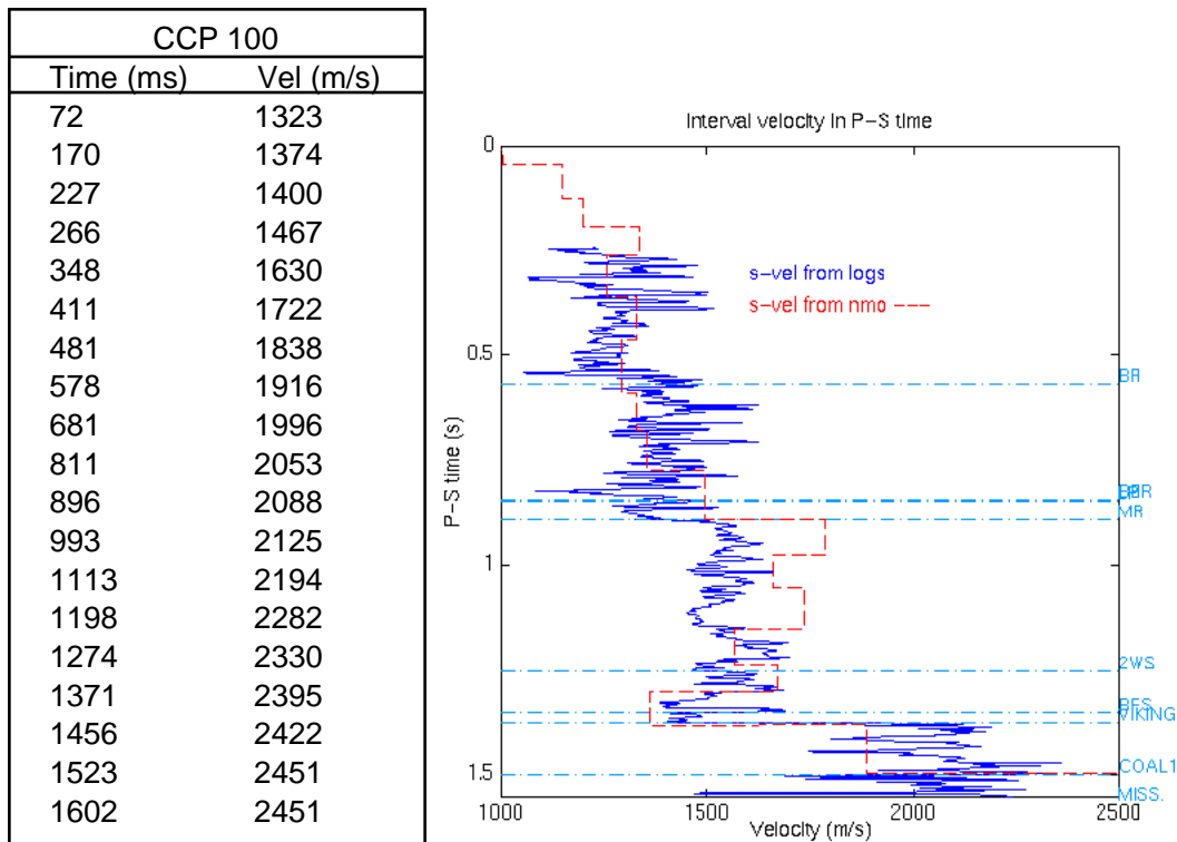
Fig. 7. a) Stacking velocity from the Blackfoot 2D - 3C. Comparison of the Dix estimate to an S-wave log from the area. The \gamma estimate is high ( \gamma = 3.25 ) due to picking the stacking velocities (a) based on large-offset NMO semblance.
