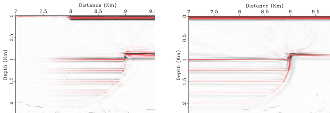
FIG. 3. RTM migrations from a usual survey (100 shots) and the complete survey (1000 shots).
