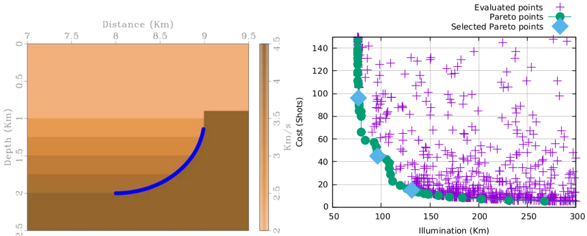
FIG. 1. Left: Velocity model with the region of interest is highlighted. Right: Pareto Front obtained from the bi-objective optimization.
