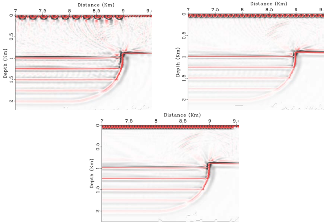
FIG. 2. RTM migrations of the selected surveys of Figure 1 right. Above are S1 with 15 shots and S2 with 45 shots. Below is S3 with 96 shots.
