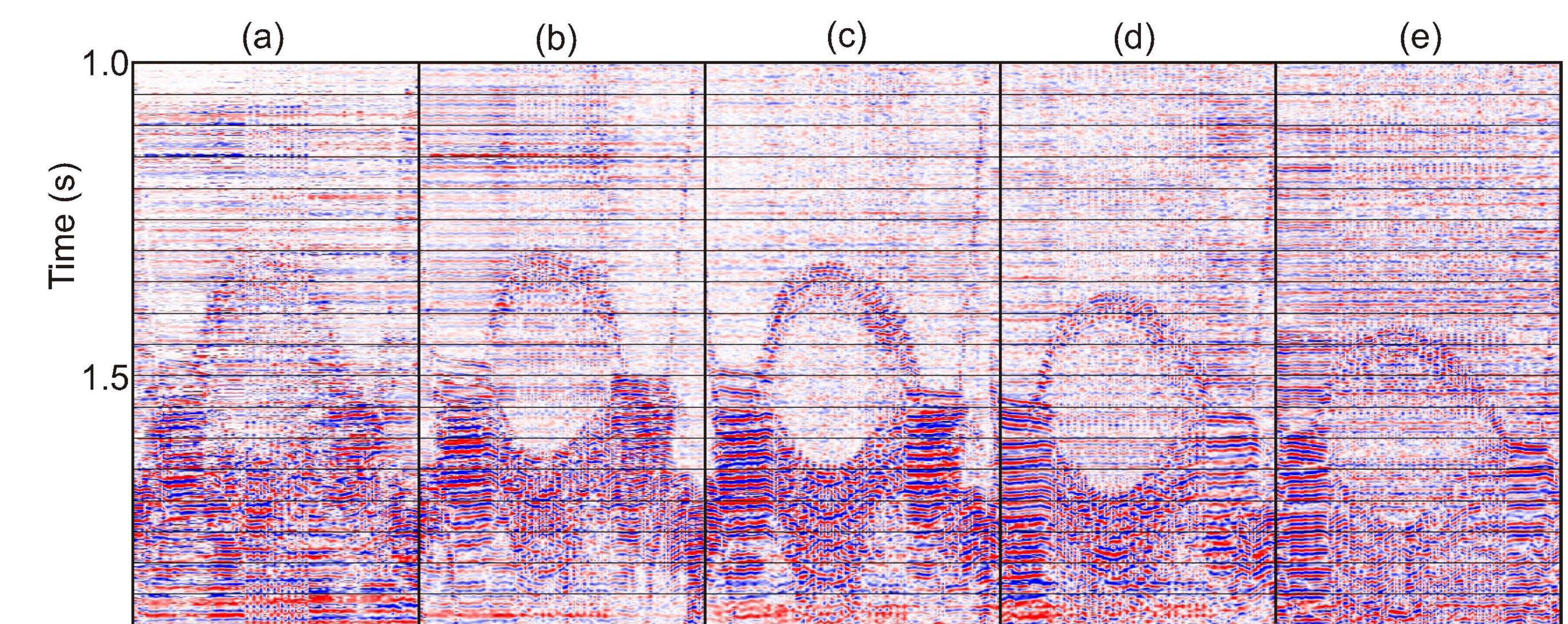
FIG. 4. Source-receiver offset gathers of north-south inline 4 over the C limb of the C-D anticline (Figure 1). The offsets are (a) 100 m, (b) 300 m, (c) 500 m, (d) 700 m and (e) 900 m.
