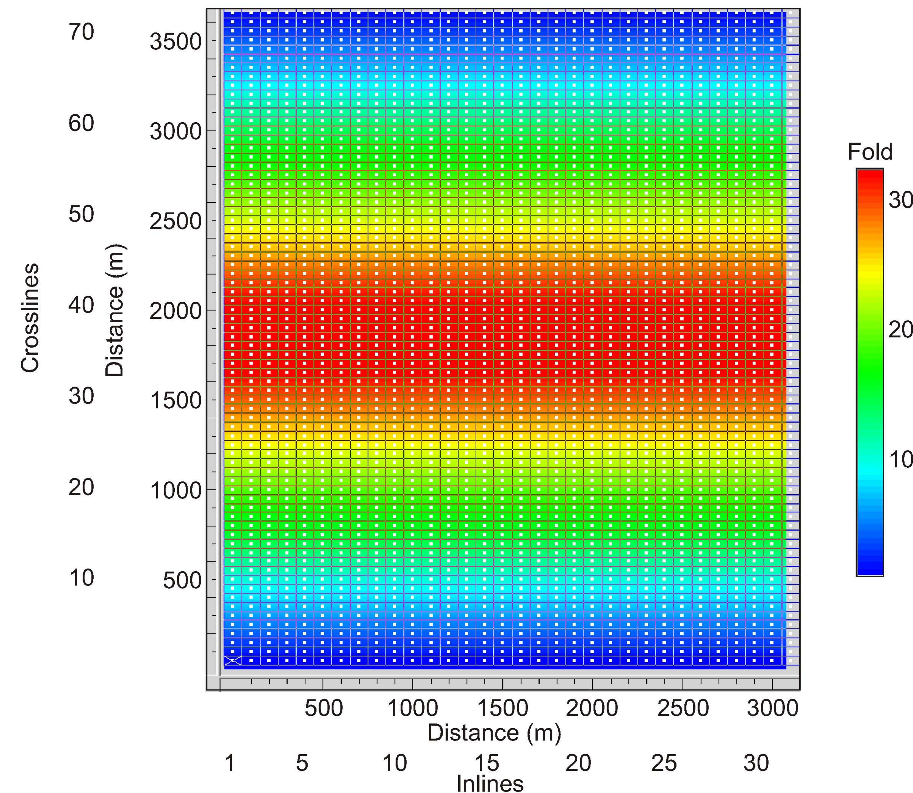
FIG. 2. Fold of the marine 3D survey.
