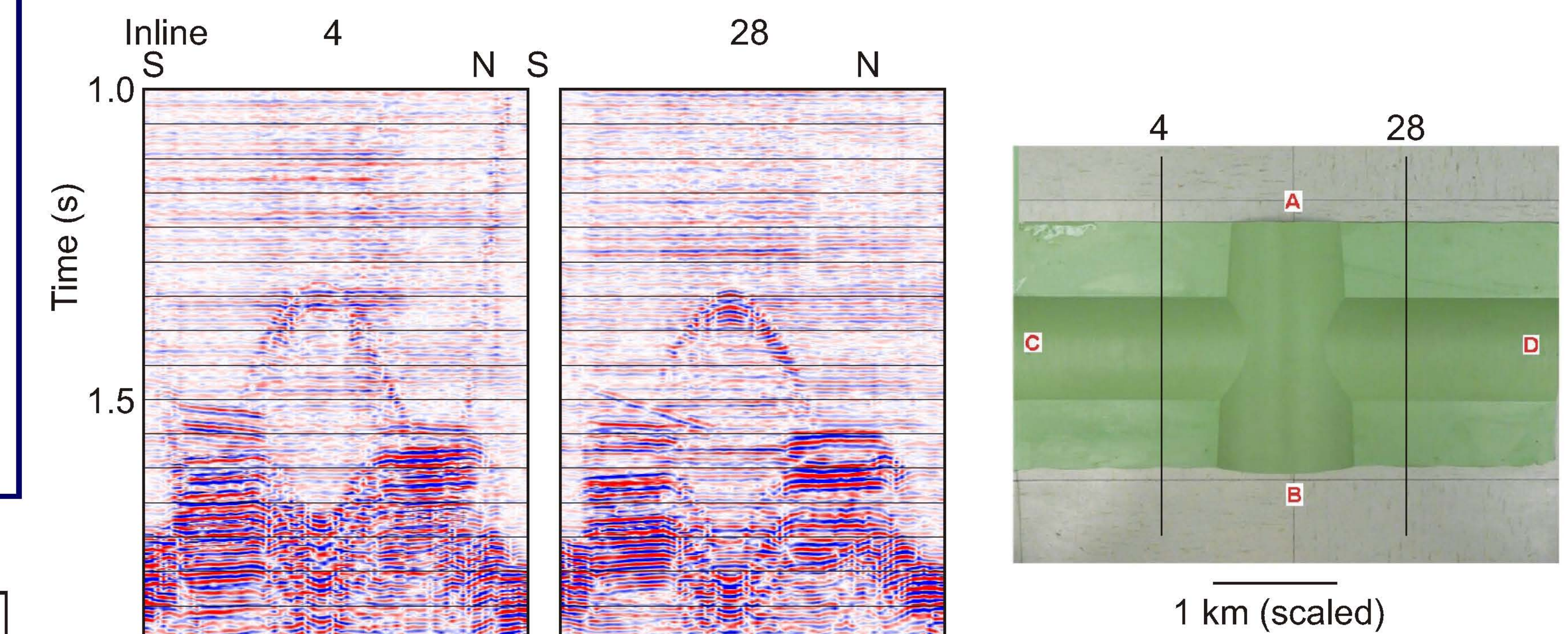
FIG. 5. North-south inlines 4 and 28 which cross the west and east limbs, respectively, of the C-D anticline. Source-receiver offsets of 300-900 m were included in these stacks.
