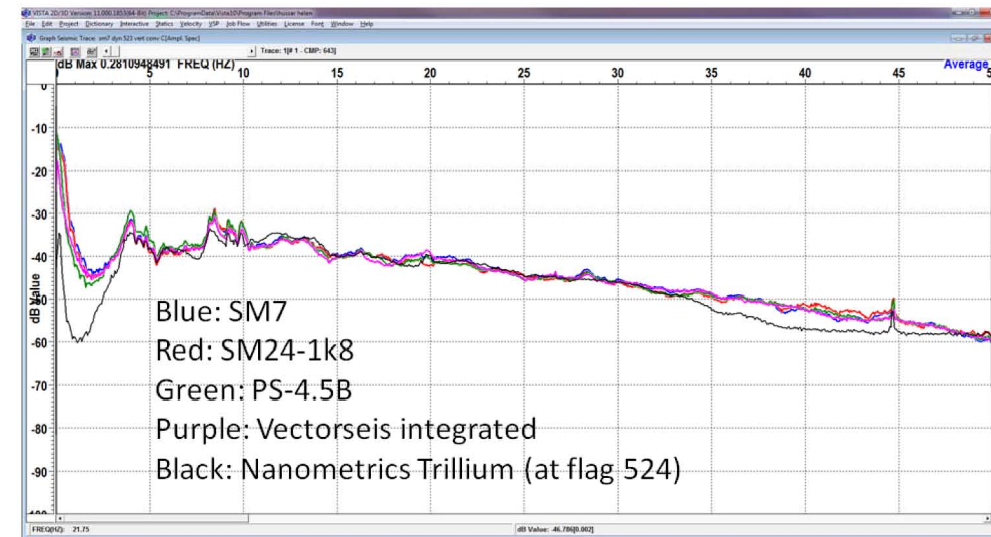
Spectra for receiver gathers at flag 523 after low frequency recovery
