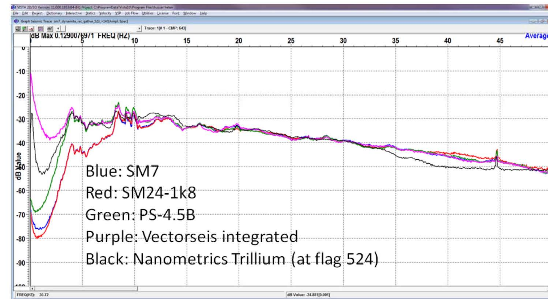
Spectra for receiver gathers at flag 523 with offset >140m
