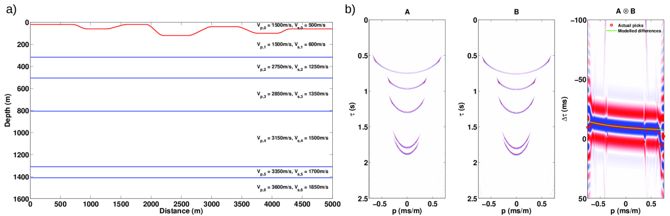
Figure 2. a) Velocity model used to compute synthetic converted-wave traces via ray-tracing. b) Crosscorrelation between reference \tau - p gather (A) and \tau - p data at receiver location x=2020m (B). Modelled and picked \tau -differences are overlaid on the crosscorrelation panel.
