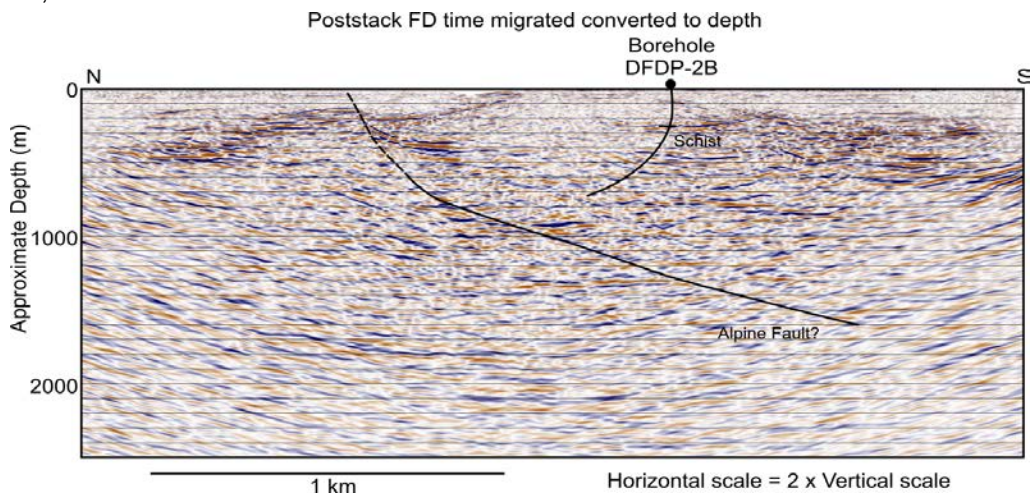
Figure 2. Top 2500 m of the depth-converted poststack time migrated section with the location of the DFDP-2B borehole and our interpretation of the Alpine Fault.
