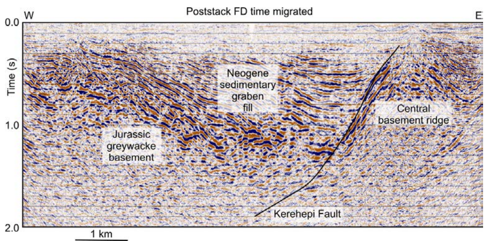
Figure 3. Interpretation of the Hauraki line with the main structural features annotated.
