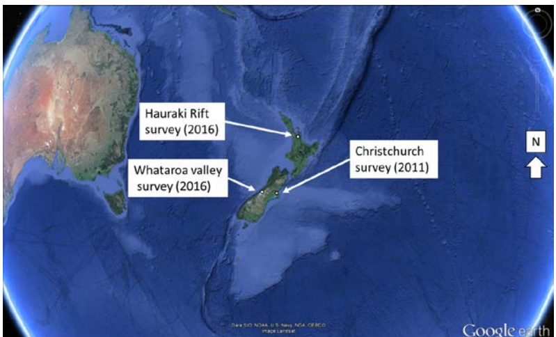
Figure 1. Location of New Zealand seismic surveys CREWES has participated in (Google Earth, 2016). Data: SIO, NOAA, U.S. Navy, NGA, GEBCO. Image: Landsat. The Christchurch survey is described by Lawton et al., 2012 and Lawton et al., 2013.
