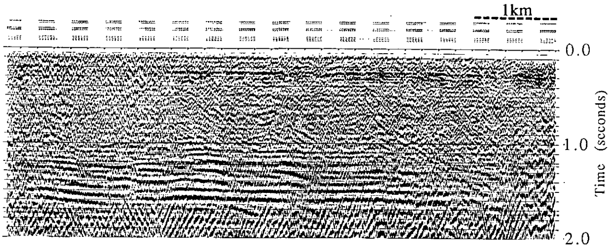
Fig. 4a: Brute stack section of the radial (P-SV) component data from Line EUE001, Slave Lake, northern Alberta.
