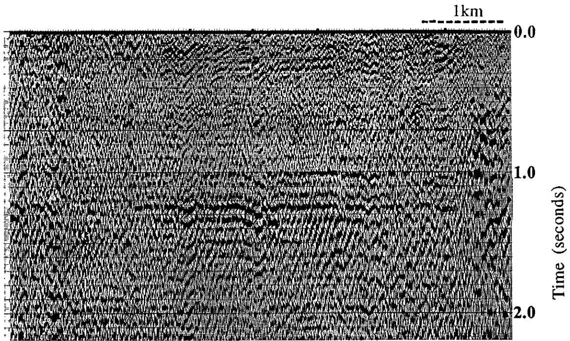
Fig. 10a: Common-receiver stacked section for the radial (P-SV) component data with P-SV refraction statics applied.
