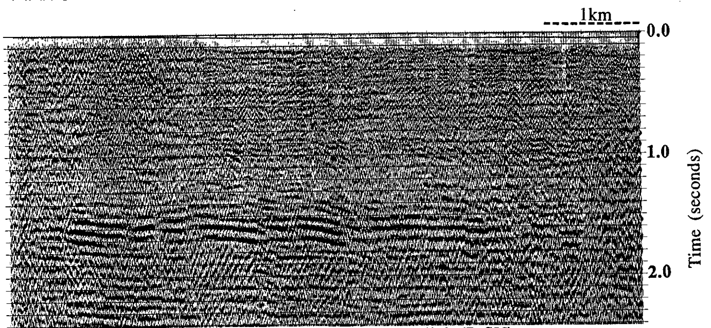
Fig. 11a: Brute stack section of the radial (P-SV) component data from Line EUE001, Slave Lake, northern Alberta.
