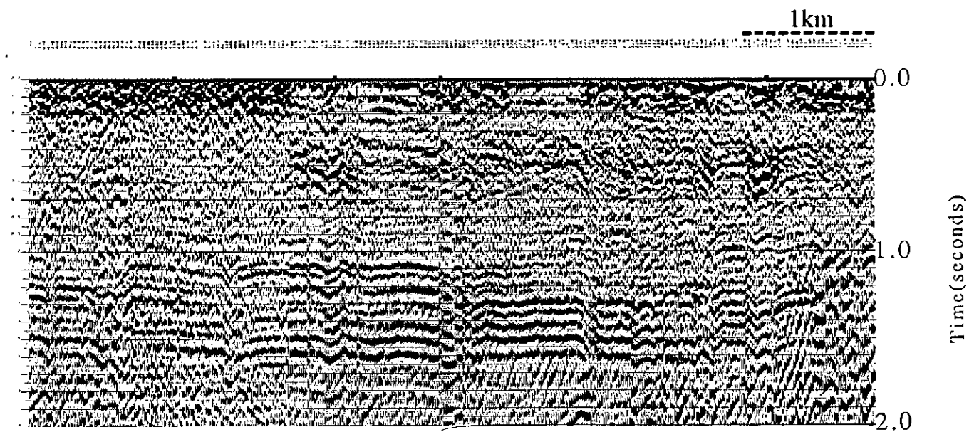
Fig. 3b: Common-receiver stack section for the Radial (P-SV) component data.
