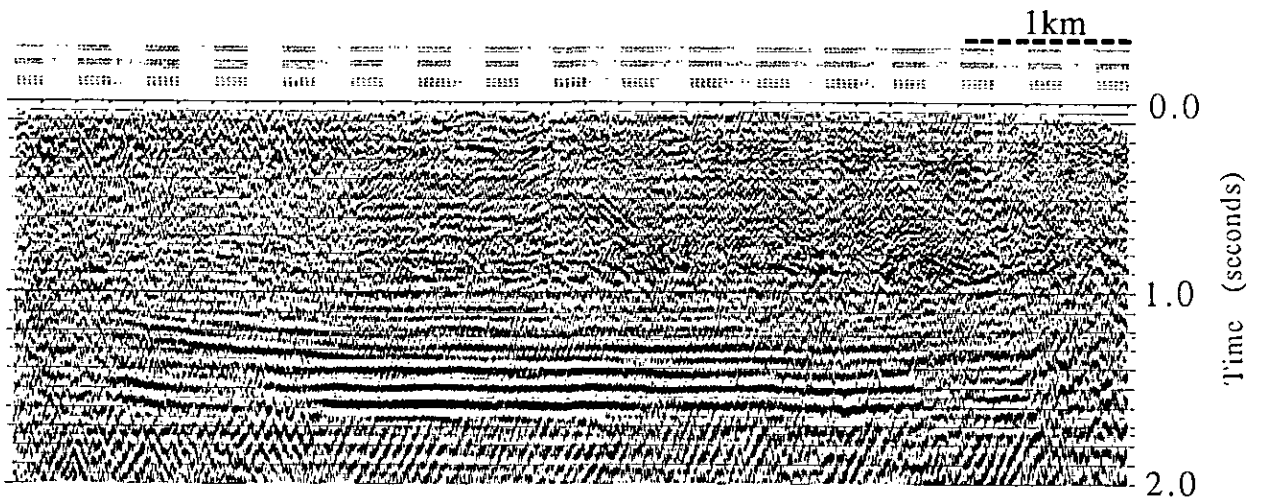
Fig. 4b: Radial (P-SV) component stack section with final statics applied.
