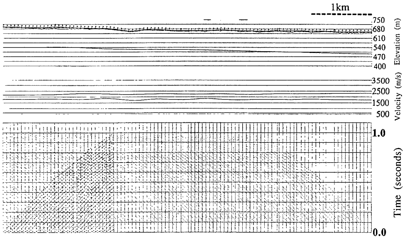
Fig. 9b: P-wave refraction picks and solution of P-wave thicknesses and velocities of the near surface.
