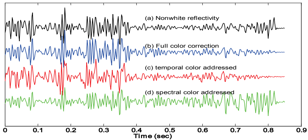
FIG. 10. Reflectivity estimations: (a) true reflectivity; (b) full color correction estimation; (c) temporal color addressed estimation; (d) spectral color addressed estimation.
