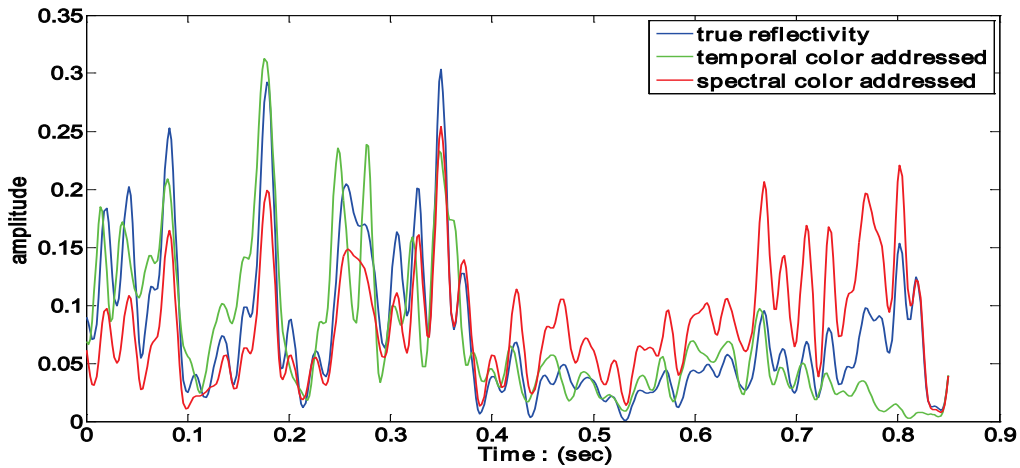
FIG. 12. Envelopes of the reflectivity series shown in figure 10.
