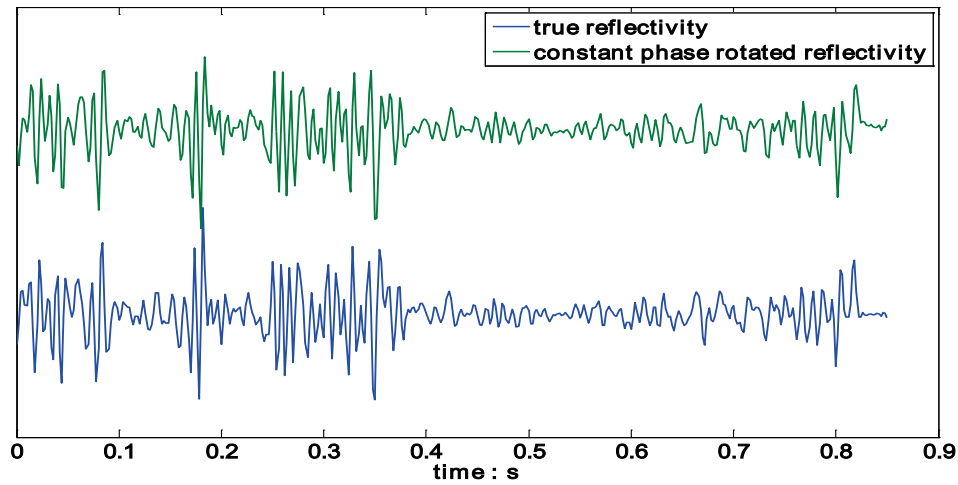
FIG. 3. A true reflectivity series and its' 60 degree rotated version.
