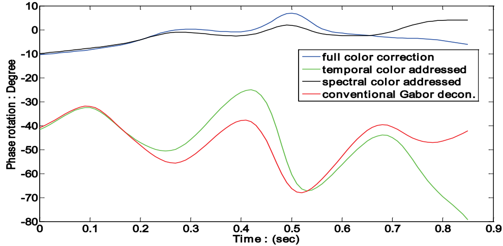
FIG. 11. Phase rotation of reflectivity estimations shown in figure 10.
