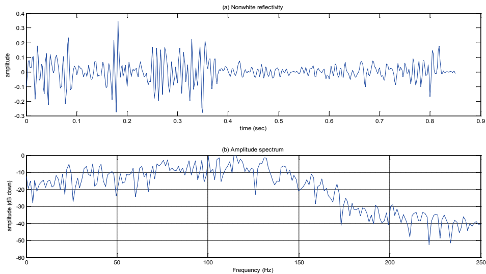
FIG. 1. (a) Nonwhite reflectivity calculated from a well log. (b) The amplitude Fourier spectrum of nonwhite reflectivity.
