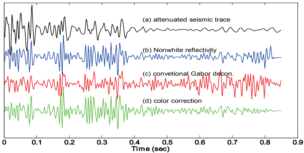
FIG. 5. Gabor deconvolution with a frequency band of 10-15 Hz. (a) Synthetic attenuated trace. (b) Nonwhite reflectivity. (c) Gabor deconvolved trace without color correction. (d) Gabor deconvolved trace with color correction using a complete well log.
