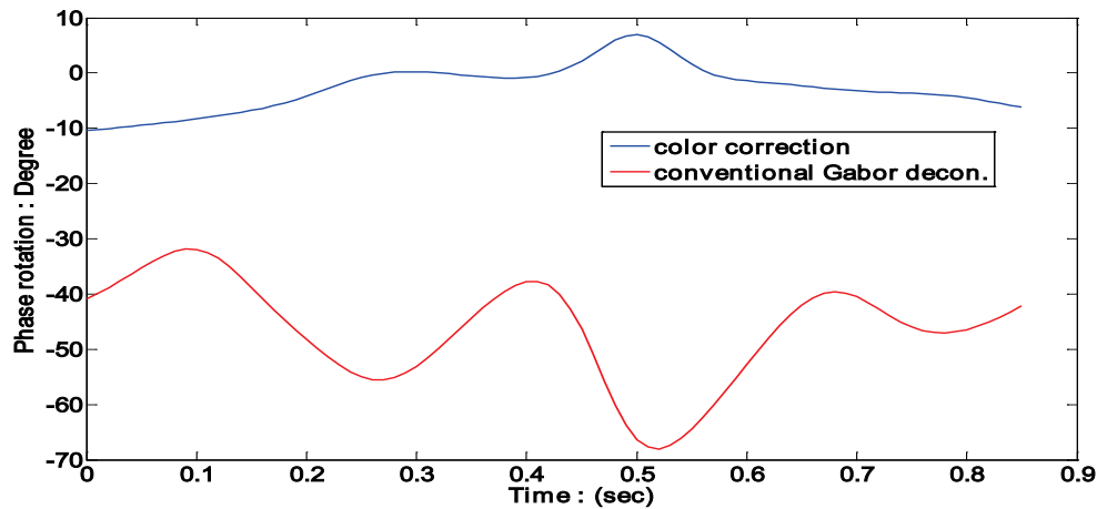
FIG. 7. Nonstationary phase rotation of the estimated reflectivity series shown in figure 5.
