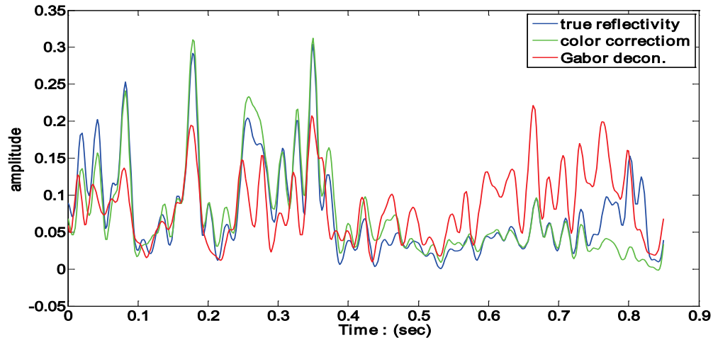
FIG. 6. Envelopes of the reflectivity series shown in figure 5.
