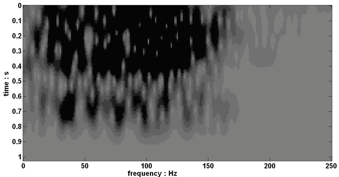
FIG. 2. Amplitude Gabor spectrum of the nonwhite reflectivity shown in Figure 1.
