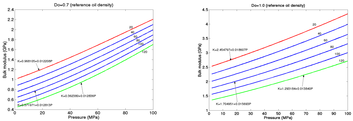
Figure 6.11 Change of oil bulk modulus with pressure. The calculation is based on equations 2.32 and 2.33 in chapter 2 and equation 20b in the paper by Batzle and Wang ( Batzle and Wang, 1992).
