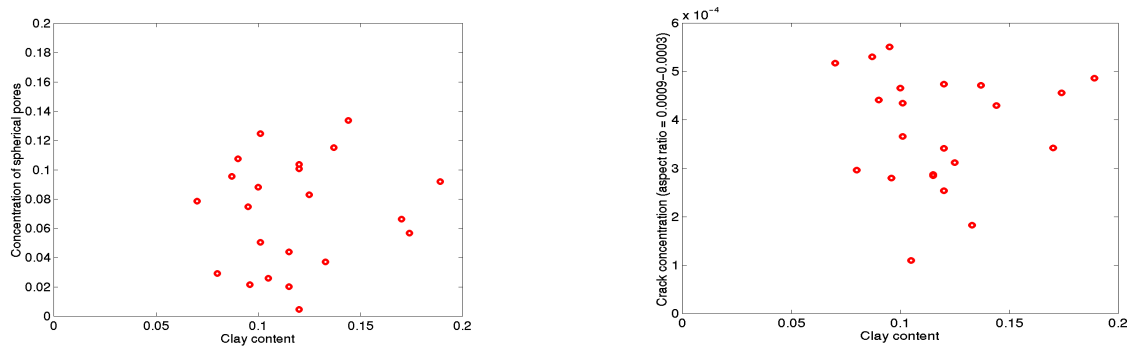
Figure 3.24 Plot of clay content versus concentration of spherical pores and low-aspect-ratio cracks, respectively, for the second set.
