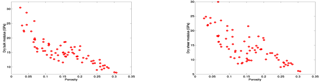
Figure 3.19 Plot of porosity versus dry bulk modulus and shear modulus at 40 MPa.
