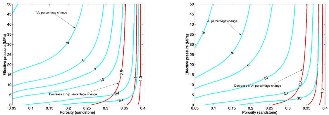
Figure 6.13 Contours of decrease in V_p (left) and AI (right) percentage changes due to a decrease of fluid bulk moduli (0.05 for water and 0.1 for oil, after water drive). The decrease in V_p
