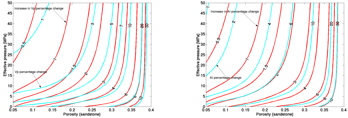
Figure 6.4 Contours of increase in the V_p (left) and AI (right) percentage changes due to an increase in water bulk modulus (to 3.1 GPa). The contour lines of the percentage changes are computed based on the same fluid properties as those in Figure 6.1. The increase in V_p percentage change is defined as (\Delta V_p/V_{p\text{-before}} * 100\%)_{\text{adjusted water bulk modulus}} - (\Delta V_p/V_{p\text{-before}} * 100\%)_{\text{original case}} . The increase in AI percentage change is defined as (\Delta AI/AI_{\text{before}} * 100\%)_{\text{adjusted water bulk modulus}} - (\Delta AI/AI_{\text{before}} * 100\%)_{\text{original case}} .
