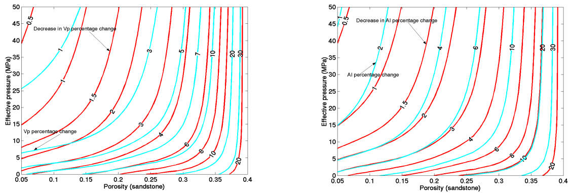
Figure 6.5 Contours of decrease in the V_p (left) and AI (right) percentage changes due to a decrease in water bulk modulus (to 1.4 GPa). The contour lines of the percentage changes are computed based on the same fluid properties as those in Figure 1. The decrease in V_p percentage change is defined as (\Delta V_p/V_{p\text{-before}} * 100\%)_{\text{original case}} - (\Delta V_p/V_{p\text{-before}} * 100\%)_{\text{adjusted water bulk modulus}} . The decrease in AI percentage change is defined as (\Delta AI/AI_{\text{before}} * 100\%)_{\text{original case}} - (\Delta AI/AI_{\text{before}} * 100\%)_{\text{adjusted water bulk modulus}} .
