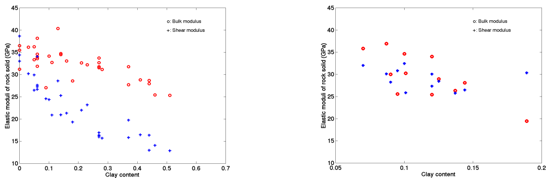
Figure 3.1 Elastic moduli of rock solid versus clay content for the samples from Han et al. (1986) on the left and from Khaksar et al. (1999) on the right. Porosity ranges from 10% to 20%.
