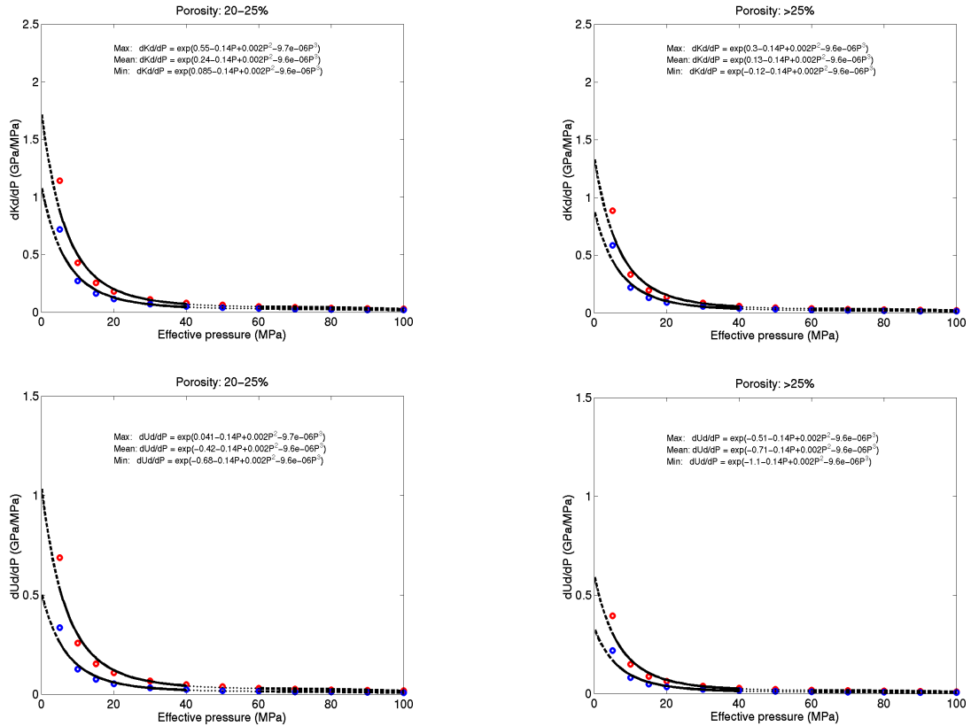
Figure 4.3 Rate of change of dry elastic moduli with effective pressure. The range with data from both sets of samples is represented by the solid lines; the dotted lines are only with the data from the second set; the dashed lines are extrapolation.
