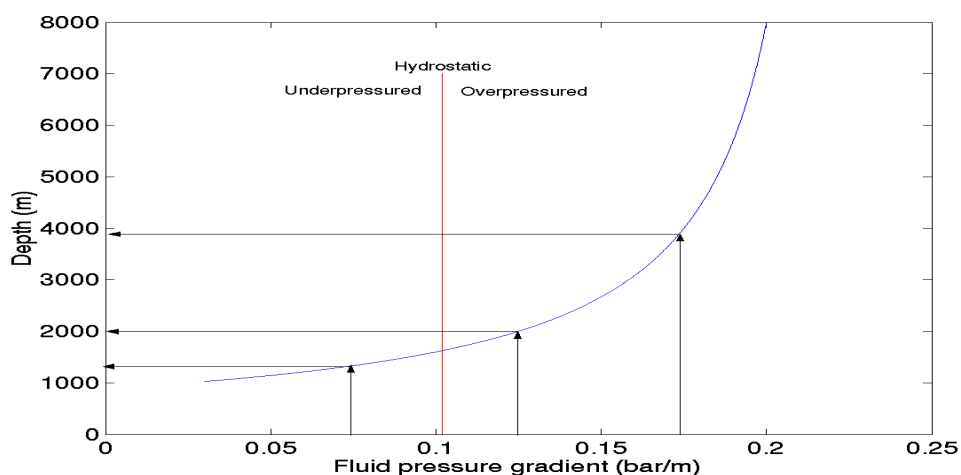
Figure 6.26 Change of the depth with the fluid pressure gradient at a given effective pressure (20 MPa). Assume S_{\text{grd}} = 0.225 \text{ bar/m} ( 2.3 \cdot 10^3 \text{ kg/m}^3 \cdot 9.8 \text{ m/s}^2 / 10^5 ).
