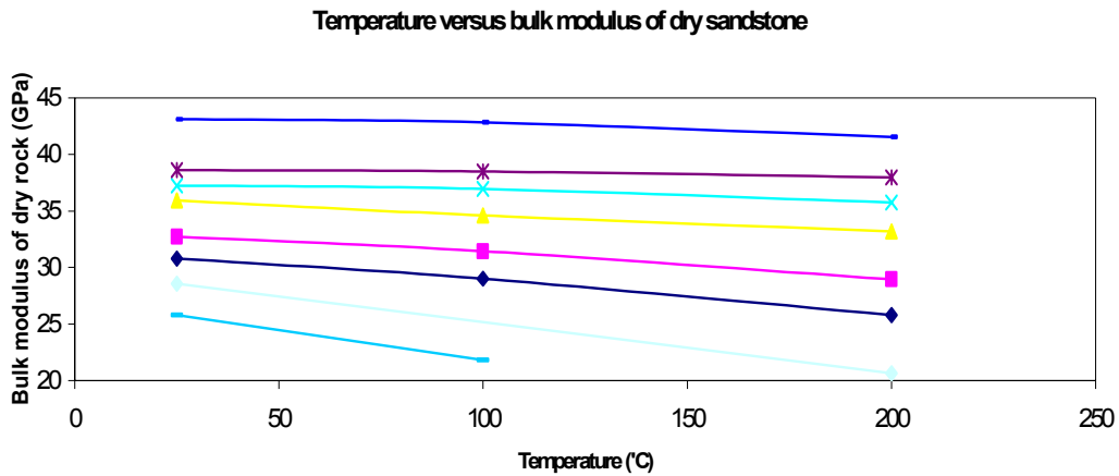
Figure 5.1 Bulk moduli versus temperature for sandstone (after Carmichael, 1989)
