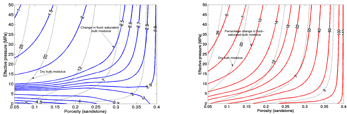
Figure 6.1 Contours of the absolute change and the percentage change in fluid-saturated bulk modulus. The dotted lines are dry bulk modulus. The absolute change of the fluid-saturated bulk modulus is defined as \Delta K = K_{\text{after}} - K_{\text{before}} , where K_{\text{after}} and K_{\text{before}} are the fluid-saturated bulk modulus after and before water drive, respectively. The percentage change is \Delta K / K_{\text{before}} * 100\% . Fluid properties are assumed: before production, D_o = 0.749(\text{g}/\text{cm}^3) , K_o = 0.67 (GPa), S_o = 75\% , D_w = 1.089(\text{g}/\text{cm}^3) , K_w = 2.38 (GPa), S_w = 25\% ; after water drive, D_o = 0.749(\text{g}/\text{cm}^3) , K_o = 0.67 (GPa), S_o = 15\% , D_w = 1.089(\text{g}/\text{cm}^3) , K_w = 2.38 (GPa), S_w = 85\% .
