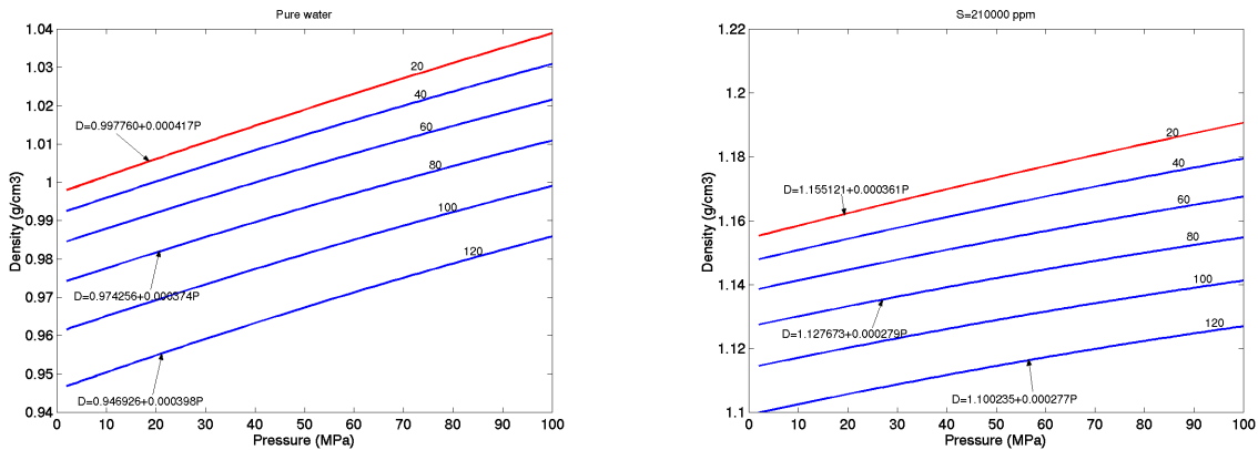
Figure 6.8 Change of water density with pressure. The calculation is based on equations 2.28 and 2.29.
