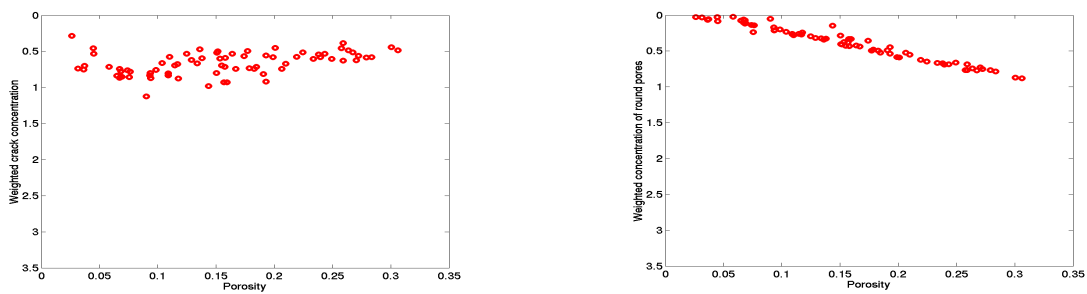
Figure 3.18 Plot of total porosity versus weighted concentration of spherical pores (right) and weighted crack concentration (left) at 40 MPa.
