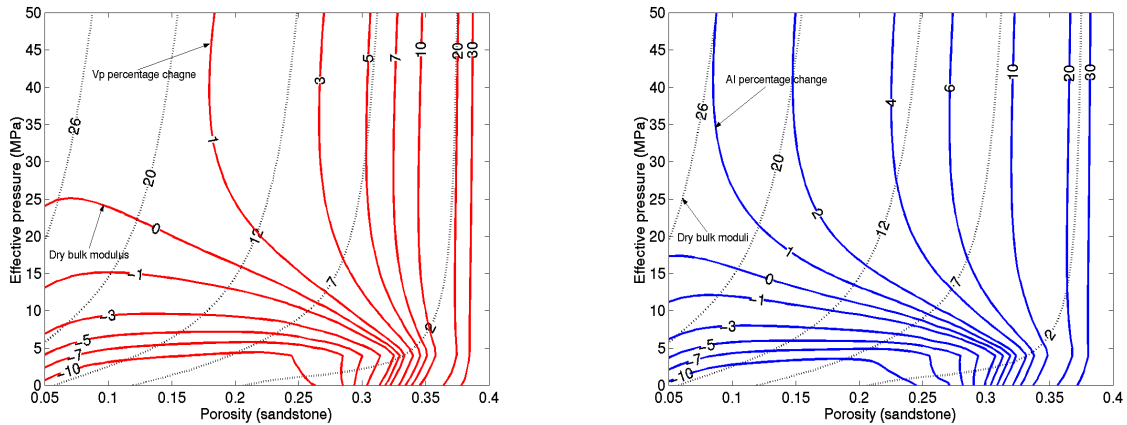
Figure 6.16 Contours of V_p and AI percentage changes. V_p percentage change is defined as \Delta V_p / V_{p\text{-before}} * 100\% . AI percentage change is defined as \Delta AI / AI_{\text{before}} * 100\% . Fluid properties are assumed: before production, D_o=0.749(\text{g}/\text{cm}^3) , K_o=0.67 (GPa), S_o=75\% , D_w=1.089(\text{g}/\text{cm}^3) , K_w=2.38 (GPa), S_w=25\% ; after water injection, D_o=0.787(\text{g}/\text{cm}^3) , K_o=1.01 (GPa), S_o=15\% , D_w\text{-inj}=1.089(\text{g}/\text{cm}^3) , K_w\text{-inj}=2.38 (GPa), S_w\text{-inj}=60\% , D_w\text{-irr}=1.115(\text{g}/\text{cm}^3) , K_w\text{-irr}=2.60 (GPa), S_w\text{-irr}=25\% .
