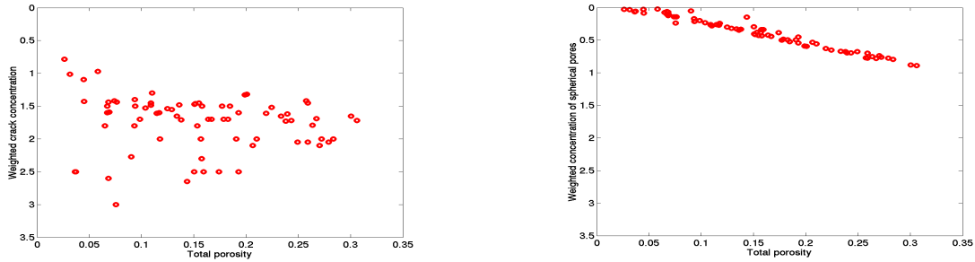
Figure 3.12 Plot of total porosity versus weighted concentration of spherical pores (right) and weighted crack concentration (left).
