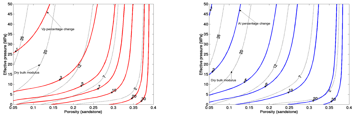
Figure 6.3 Contours of V_p and AI percentage changes. Fluid properties are the same as those in Figure 6.1. The V_p percentage change is defined as \Delta V_p / V_{p\text{-before}} * 100\% = (V_{p\text{-after}} - V_{p\text{-before}}) / V_{p\text{-before}} * 100\% , where V_{p\text{-after}} and V_{p\text{-before}} are the primary wave velocity after and before water drive, respectively (the same below). The AI percentage change is defined as \Delta AI / AI_{\text{before}} * 100\% = (AI_{\text{after}} - AI_{\text{before}}) / AI_{\text{before}} * 100\% , where AI_{\text{after}} and AI_{\text{before}} are the acoustic impedance after and before water drive, respectively (the same below).
