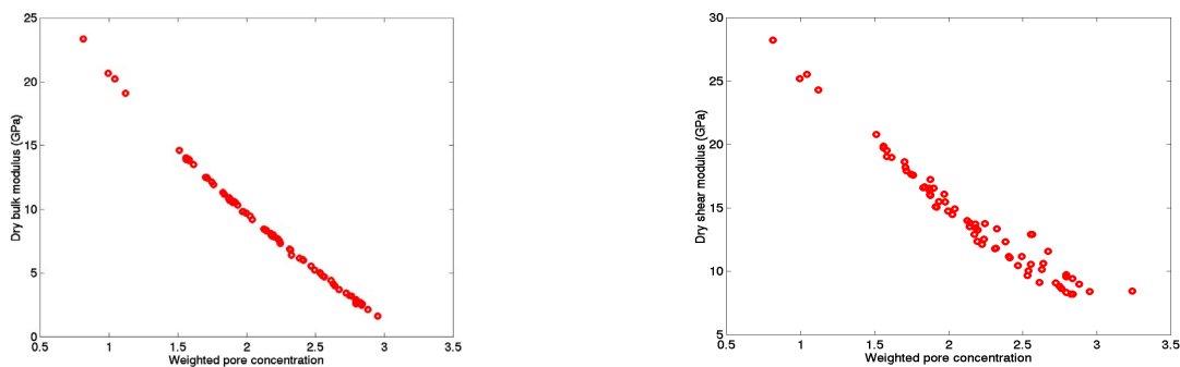
Figure 3.6 Plot of weighted concentrations versus dry elastic moduli computed based on the constant elastic moduli of rock solid ( K_s=37 GPa and \mu_s=44 GPa).
