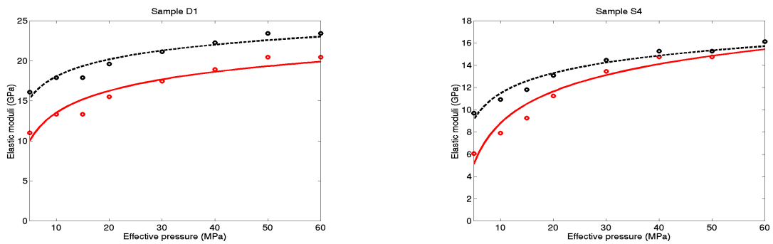
Figure 4.2 Plot of elastic moduli versus effective pressure for the second set of dry sandstones. The red and black circles are the theoretical calculations of bulk and shear moduli respectively. The red solid and black dashed lines are the corresponding regression lines.
