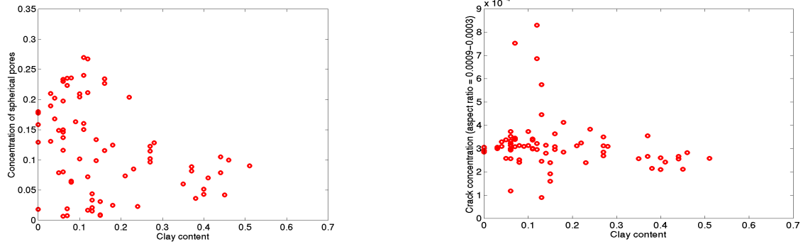
Figure 3.23 Plot of clay content versus concentration of spherical pores and low-aspect-ratio cracks, respectively, for the first set.
