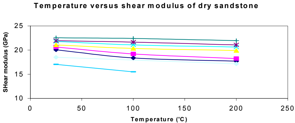
Figure 5.2 Shear moduli versus temperature for sandstone (after Carmichael, 1989)
